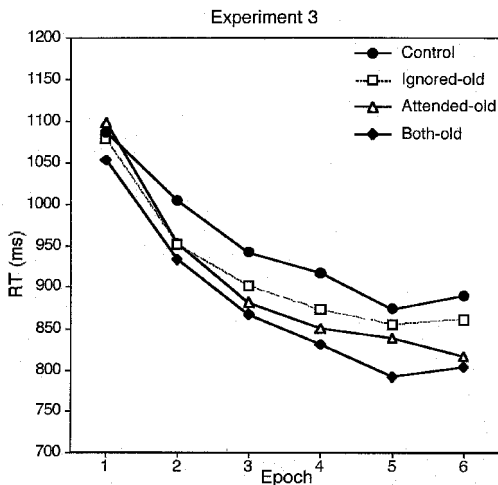
Figure 3. Mean RT data from Experiment 3.
